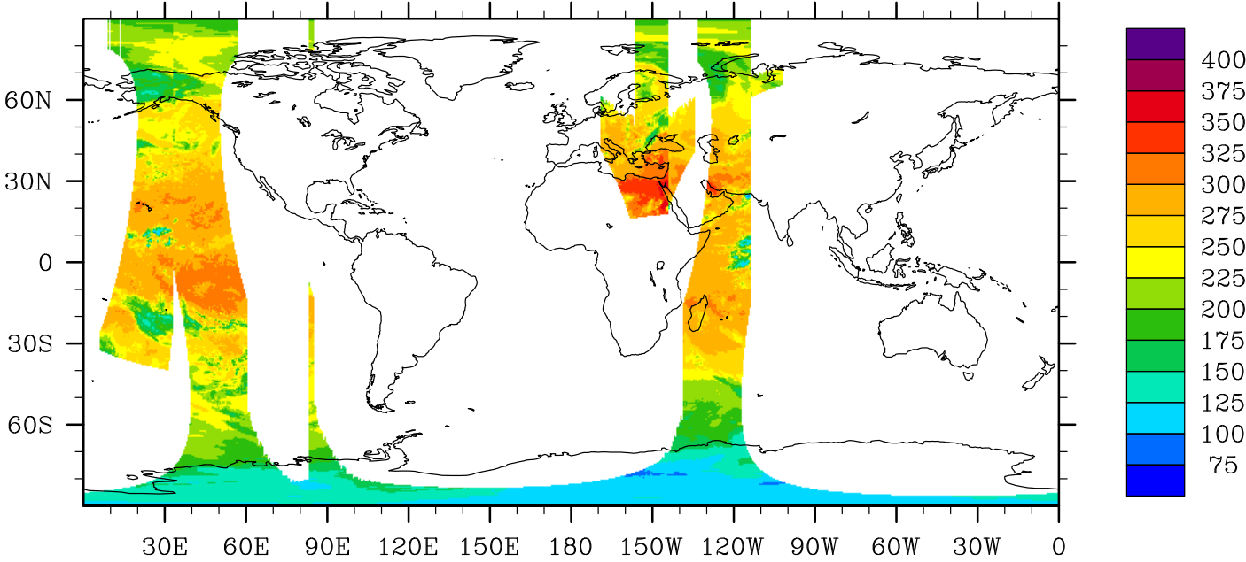
CERES LW flux at TOA
